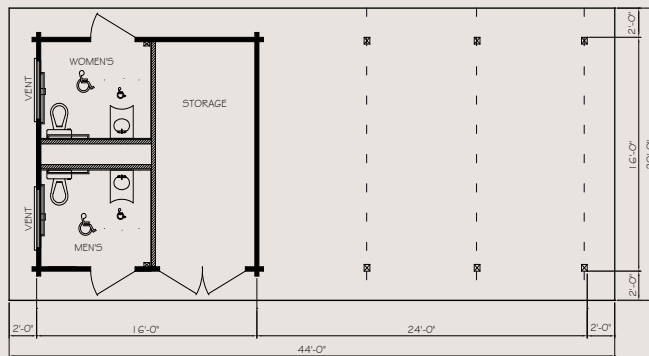
PAC 2 20' x 44' with 16' x 16' enclosed
