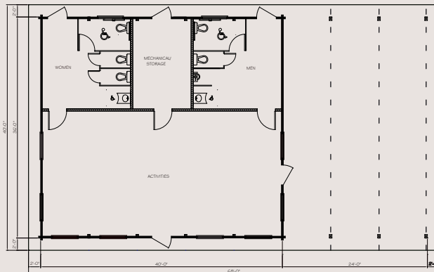
PAC 4 40' x 68' with 36' x 40' enclosed
