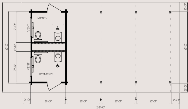
PAC 1 20' x 36' with 16' x 8' enclosed
